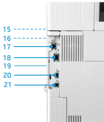
I/O panel closeup
