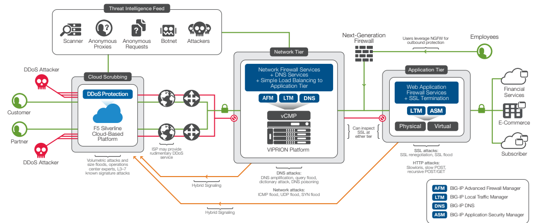
Figure 2: Divert traffic with Hybrid Signaling to Silverline DDoS Protection for cloud-scrubbing when your network is under attack, or use it to continuously scrub all traffic to prevent a DDoS attack from ever reaching your network.
