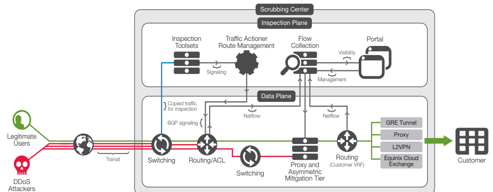
Figure 3: Silverline DDoS Protection multi-layered cloud-scrubbing technologies.
