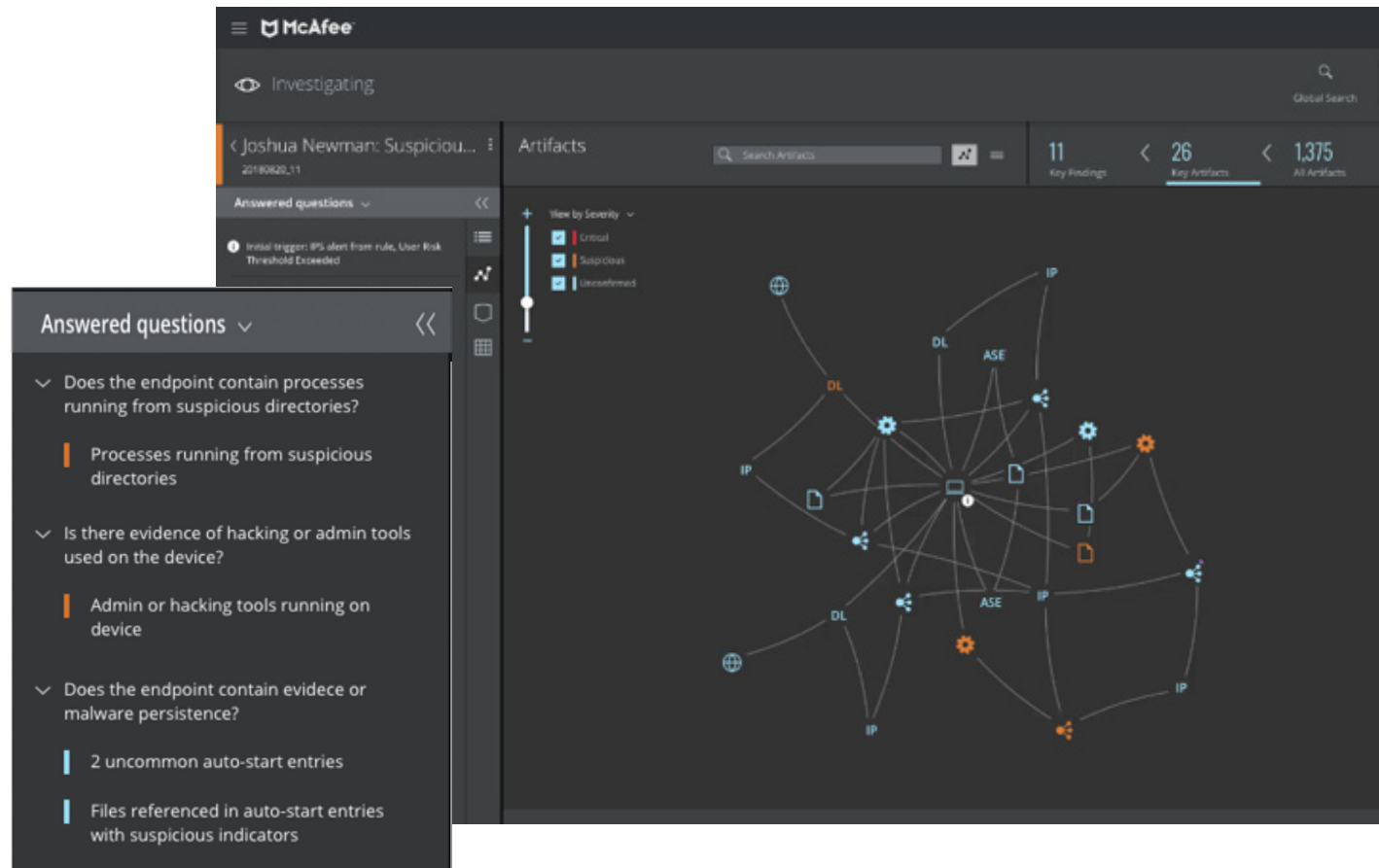
Figure 1. MVISION EDR investigates for you. It automatically collects artifacts and presents the key findings. Visualization displays relationships and speeds analyst understanding. MVISION EDR asks and answers the right questions to prove or disprove the hypotheses.
